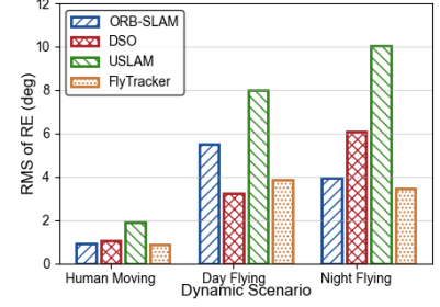
Fig. 9: RE under dynamic scenarios.
