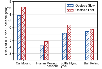
Fig. 12: ATE of obstacle motion tracking.
