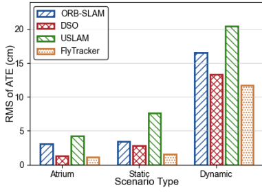
Fig. 7: Overall performance comparison.
