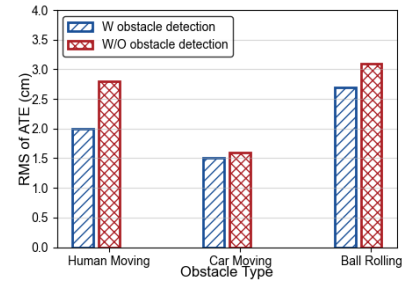
Fig. 15: ATE with and without obstacle detection.
