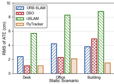
Fig. 13: ATE under static scenarios.
