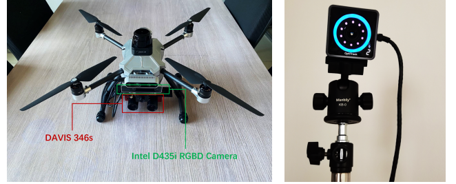
(a) drone with cameras (b) motion capture system
