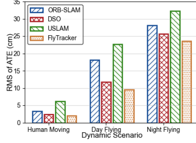
Fig. 8: ATE under dynamic scenarios.
