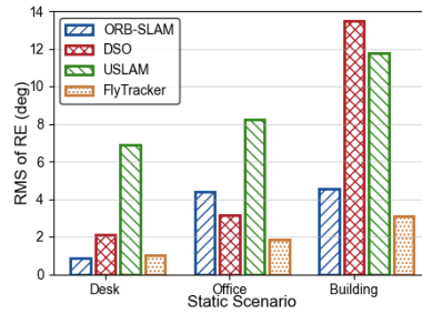
Fig. 14: RE under static scenarios.
