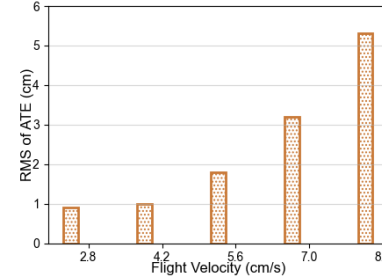
Fig. 11: ATE with flight velocities.
