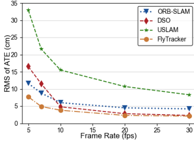
Fig. 10: ATE under different frame rates.
